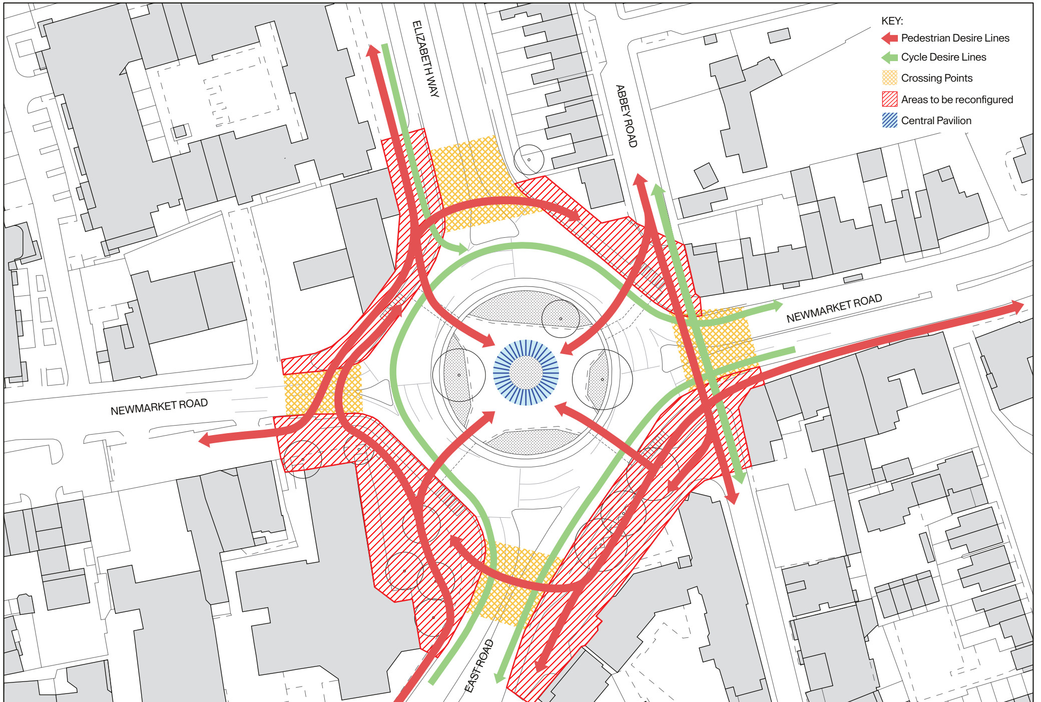
Elizabeth Way / East Road Roundabout Desire Lines Diagram
