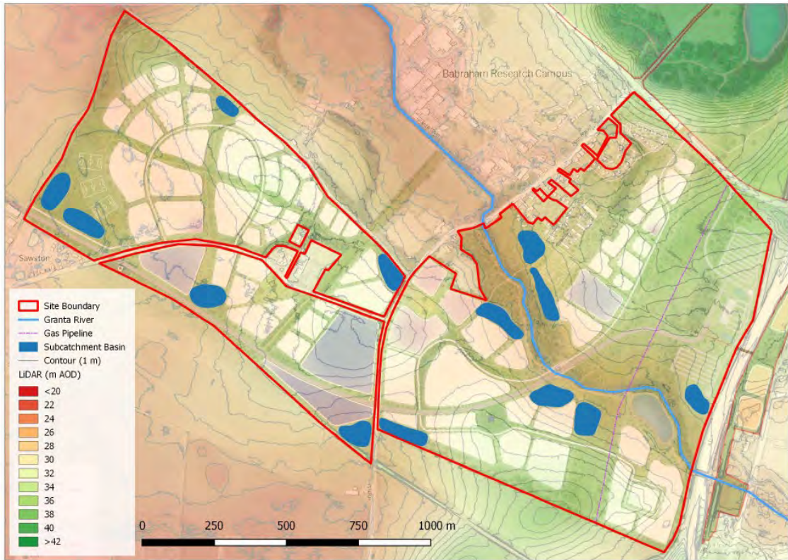
Figure 7.2: Indicative Sub-catchment Strategic Attenuation Features (Assuming No Infiltration)
