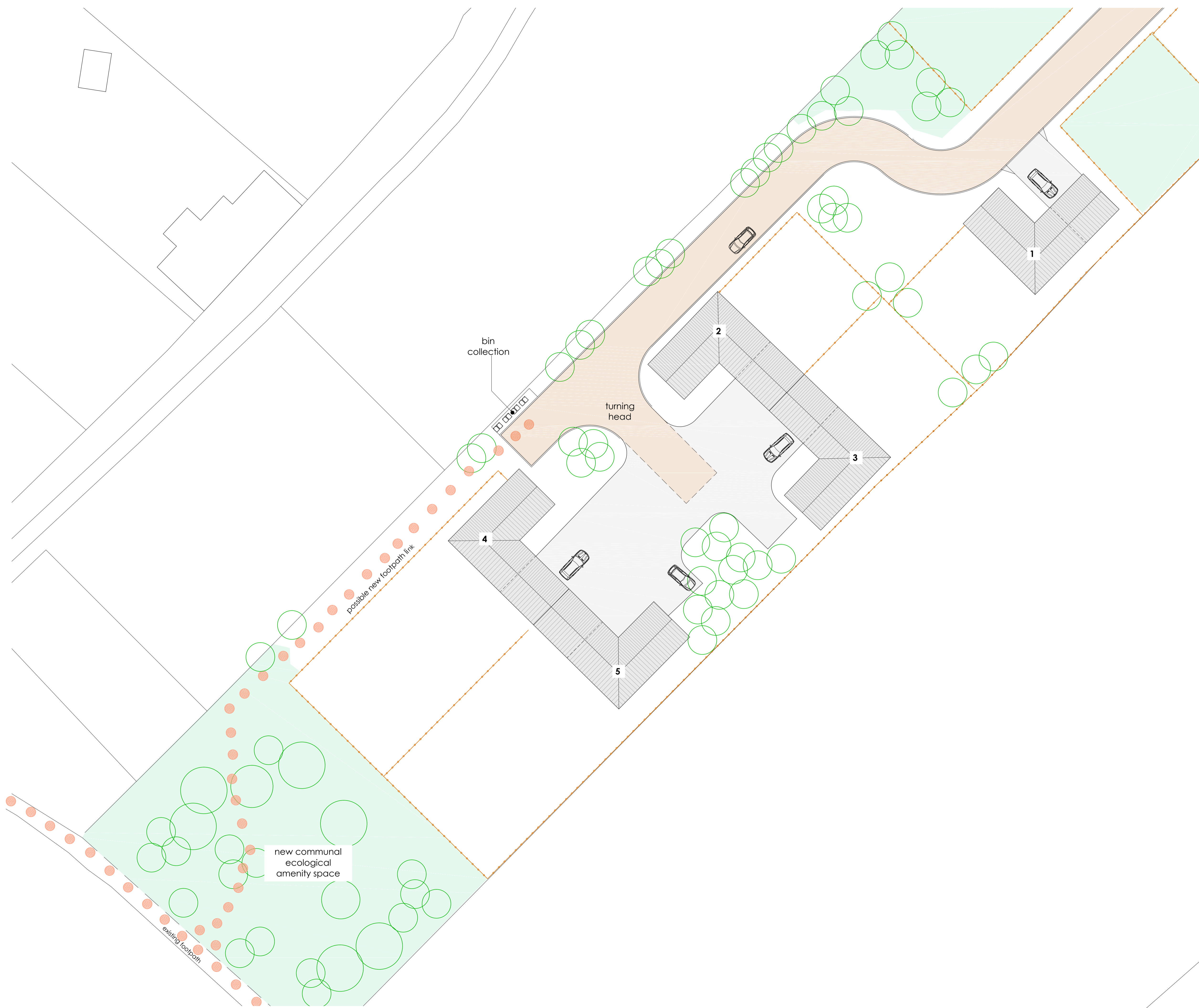
Proposed Site Layout 1:250 @ A1
